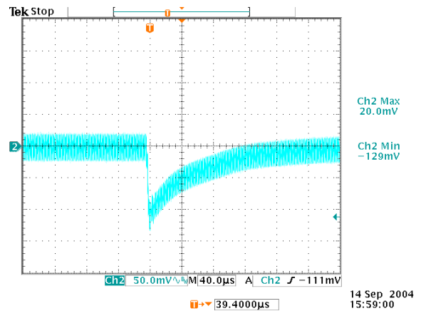
Figure 24: Typical transient response to step load change at 2.5A/μS from 50% to 100% of Io, max at 12Vin, 5.0V out (measurement with a 1uF ceramic and a 10μF tantalu)
