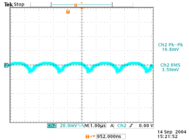
Figure 10: Output ripple & noise at 12Vin, 1.5V/4A out
