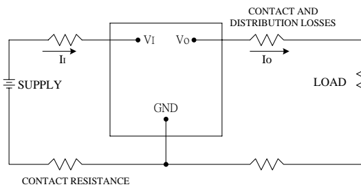
Figure 27: Output voltage and efficiency measurement test setup
