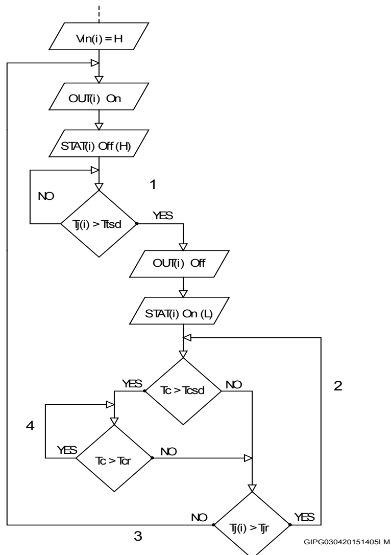
Figure 18. Thermal behavior
