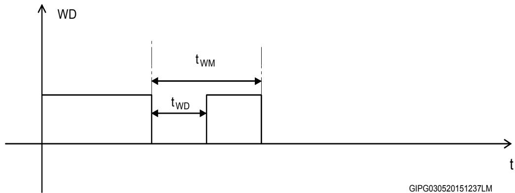
Figure 12. Watchdog reset
