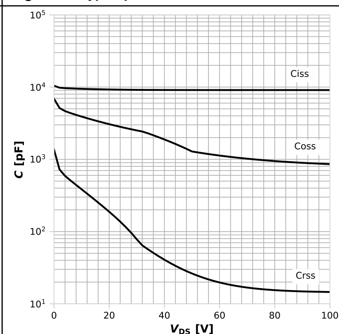
Diagram 12: Typ. capacitances
