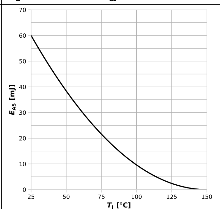
Diagram 12: Avalanche energy
