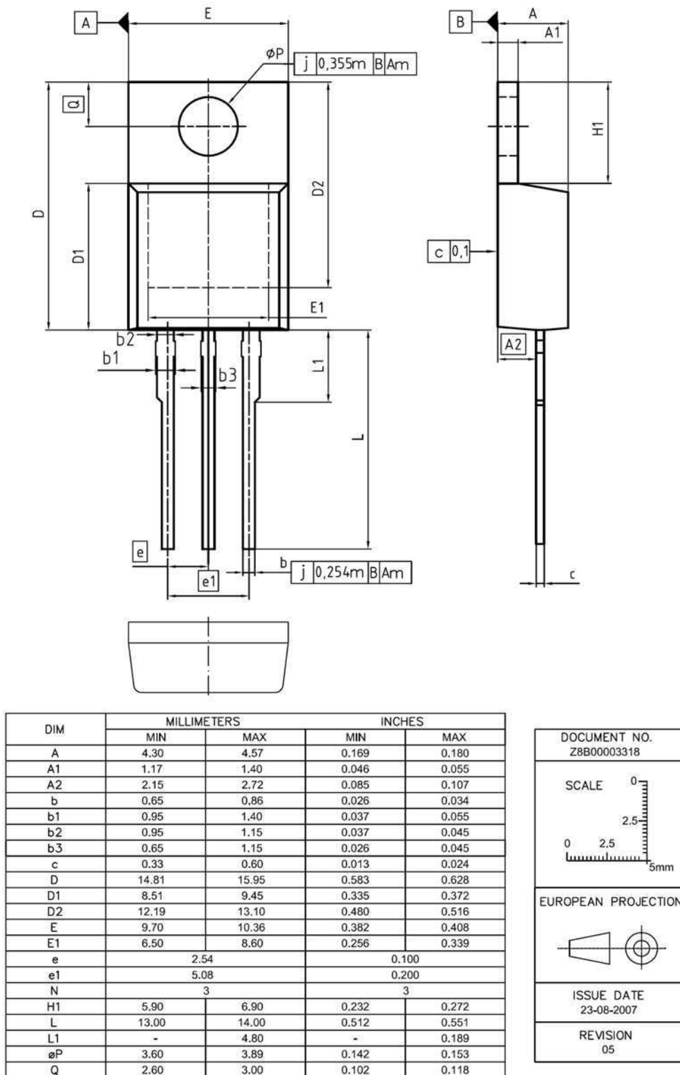
Figure 2 Outlines TO-220, dimensions in mm/inches
