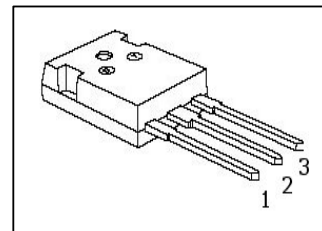
PG-TO247-3-1
