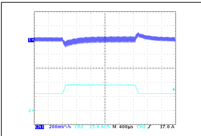
Figure 5: Output voltage response to step-change in load current (50%-75%-50% of I out (max)); dI/dt = 0.2 A/µs. Load cap: 1 µF ceramic and 15 µF tantalum capacitors. Ch 1: V out (200 mV/div), Ch 2: I out (25 A/div).
