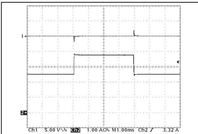
Figure 5: Output voltage response to step-change in load current (50%-75%-50% of Iout(max); dI/dt = 0.05 \text{ A}/\mu\text{s} ). Load cap: 1 \mu\text{F} ceramic capacitor. Ch 1: Vout (5 V/div), Ch 2: Iout (1 A/div).
