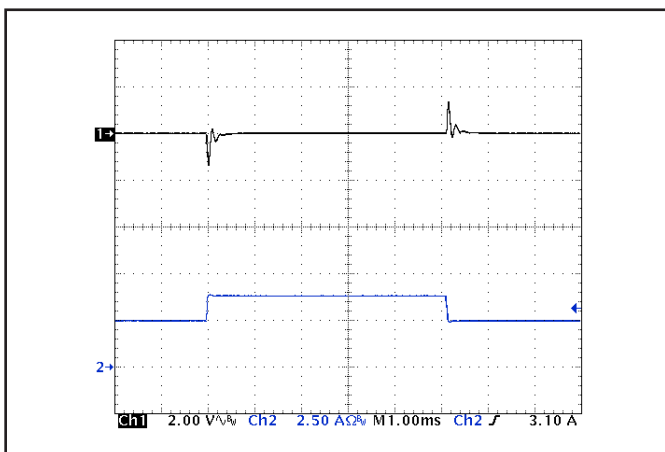
Figure 5: Output voltage response to step-change in load current (50%-75%-50% of I out (max); dI/dt = 0.05 A/μs). Load cap: 1 μF ceramic capacitor. Ch 1: V out (2 V/div), Ch 2: I out (2.5 A/div).
