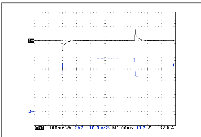
Figure 5: Output voltage response to step-change in load current (50%-75%-50% of Iout(max); dI/dt = 0.2 A/μs). Load cap: 1 μF ceramic and 15 μF tantalum capacitors. Ch 1: Vout (100 mV/div), Ch 2: Iout (10 A/div).
