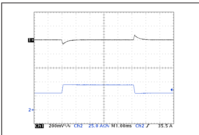
Figure 5: Output voltage response to step-change in load current (50%-75%-50% of Iout(max)); dI/dt = 0.2 \text{ A}/\mu\text{s} . Load cap: 1 \mu\text{F} ceramic and 15 \mu\text{F} tantalum capacitors. Ch 1: Vout (200 mV/div), Ch 2: Iout (25 A/div).
