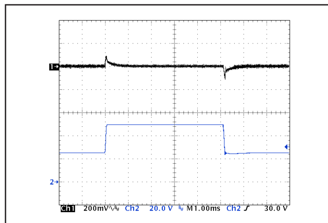
Figure 6: Output voltage response to step-change in input voltage (500 V/ms). Load cap: 100 \mu\text{F} , electrolytic output capacitance. Ch 1: Vout (200 mV/div), Ch 2: Vin (20 V/div).
