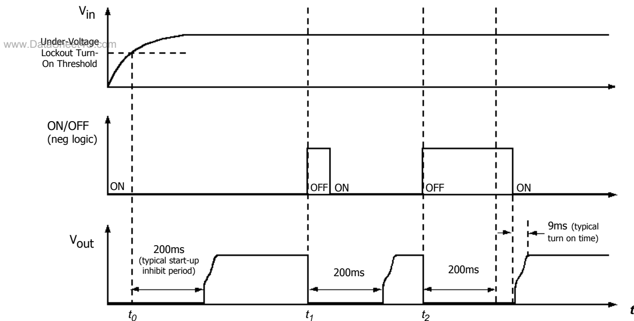
Figure F: Startup Inhibit Period (turn-on time not to scale)
