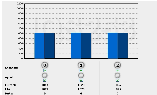
Figure A.1: DYCAL output selected on proximity, for a projected capacitive IC. Note that the IC still only enters TM (Touch Mode) when the counts exceed the touch threshold, but the DYCAL output is active after exceeding the proximity threshold.
