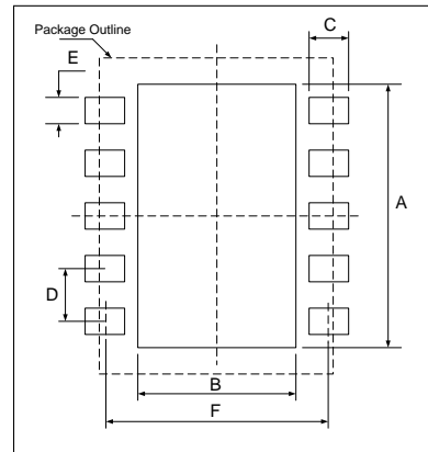
Figure 13.6: DFN-10 Footprint.
