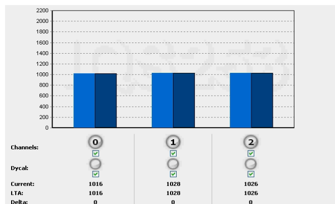
Figure A.2: DYCAL output selected on touch, for a projected capacitive IC. Note that the DYCAL output is only active when the IC enters TM (Touch Mode) when the counts exceed the touch threshold.
