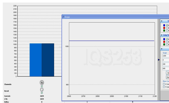
Figure A.3: Filter halt upon Touch Mode Entry, for a self capacitive IC. The LTA will halt upon proximity detection (regardless on which output DYCAL was selected). However, when a touch condition is registered, the filter will stop halting, to allow the LTA to follow the counts.
