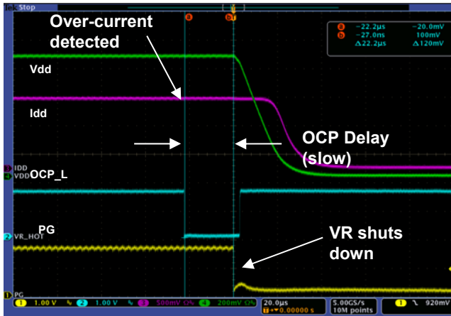
Figure 14: OCP_L (VR_HOT) assertion with OCP_TDC (Slow) threshold. OCP delay action (22usec)
