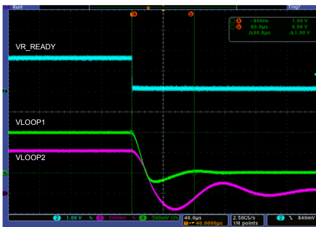
Figure 42: OVP - MOSFET latched on
