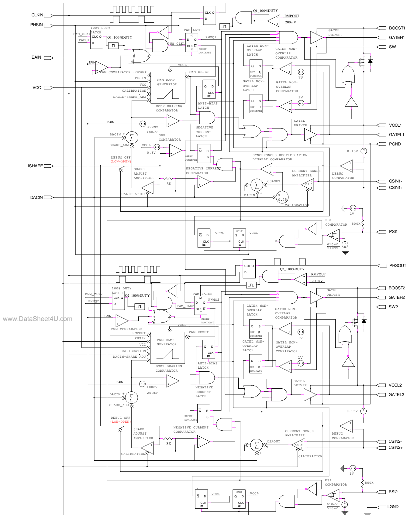
Figure 6 – IR3527 Block diagram
