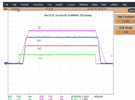
Fig. 10: Simultaneously Power up /down
