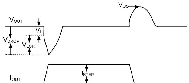
Figure 19. Typical Output Voltage Response Waveform.
