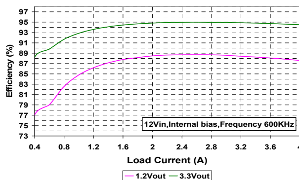
Figure 2: IR3897 Efficiency
