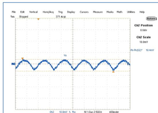
Figure 35: Output Voltage Ripple 4A Load, Ch2: V_o
