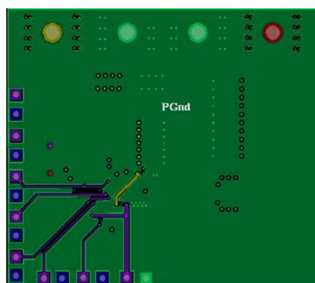
Figure 49c: IRDC3897 Demo board Layout Considerations – Mid Layer 1
