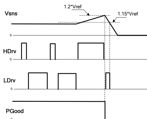
Figure 18c: Timing Diagram for OVP in non-tracking mode
