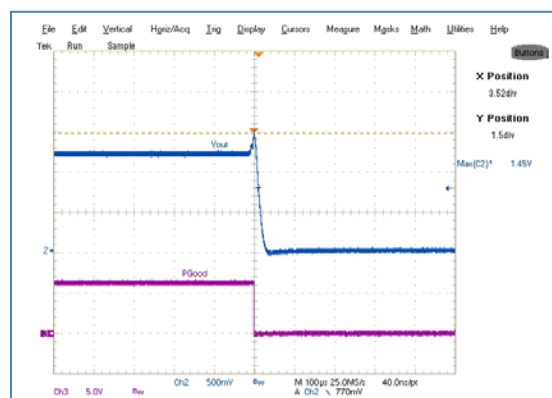
Figure 46: Over Voltage protection, Ch2: V_o , Ch3: PGood
