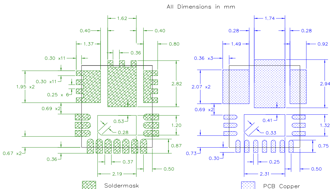
Figure 51: Solder resist
