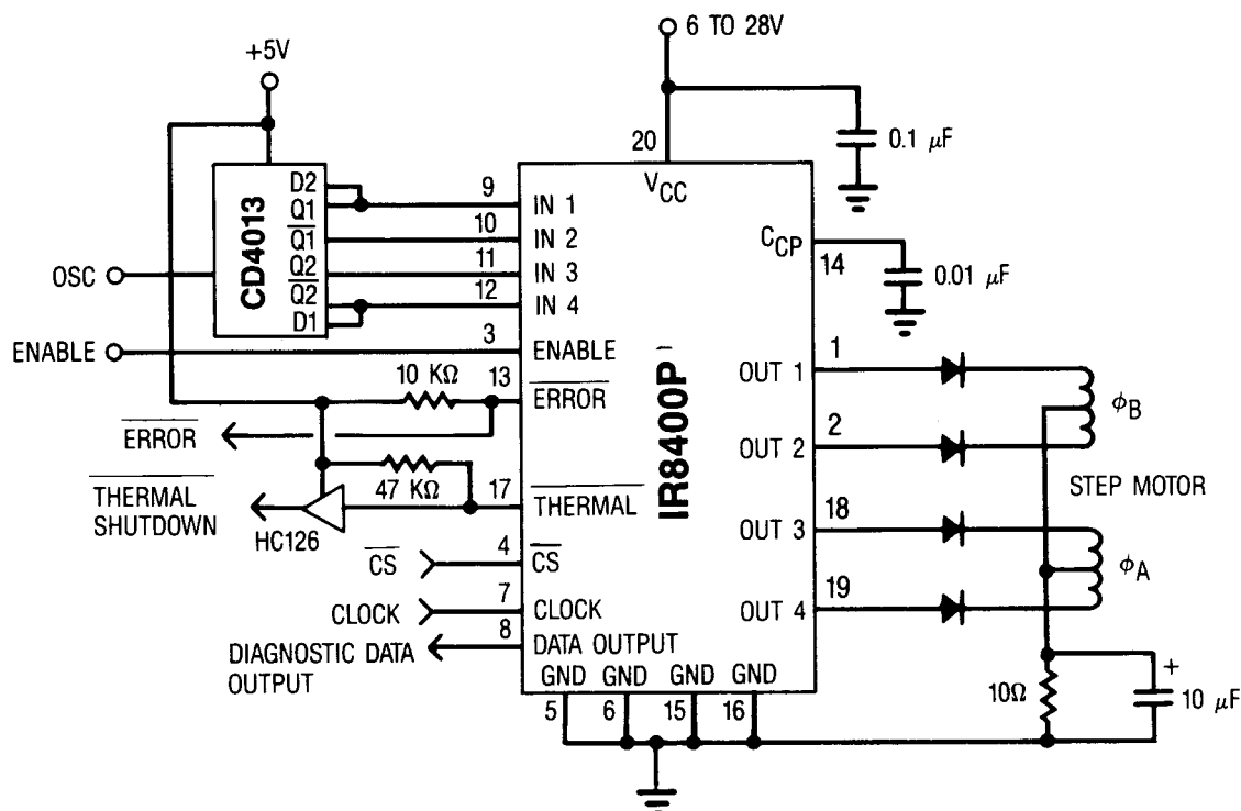
Unipolar Drive for a 2-Phase Stepper Motor
