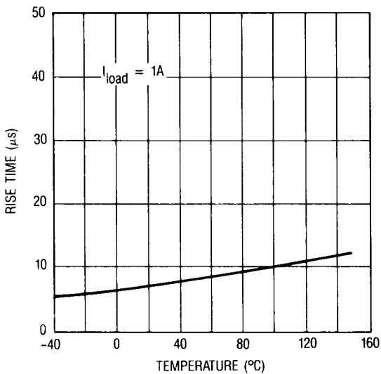
Fig. 11 — Turn ON Rise Time vs. Temperature
