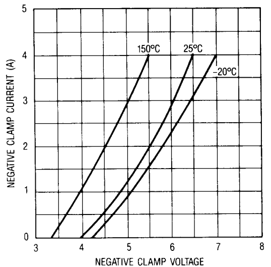
Fig. 6 — Output Voltage Characteristics vs. Temperature
