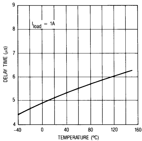
Fig. 10 — Turn ON Delay Time vs. Temperature
