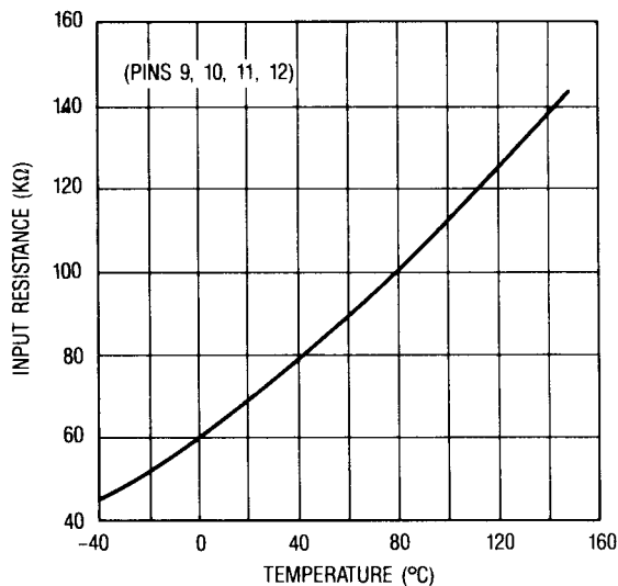
Fig. 8 — Switch Select Logic Input Resistance vs. Temperature
