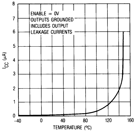
Fig. 1 — 'Sleep' Mode Supply Current vs. Temperature
