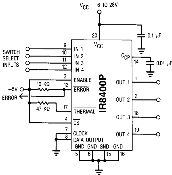
Recommended Connection if No Diagnostics are Required
