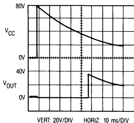
Fig. 17 — Overvoltage/Undervoltage Shutdown
