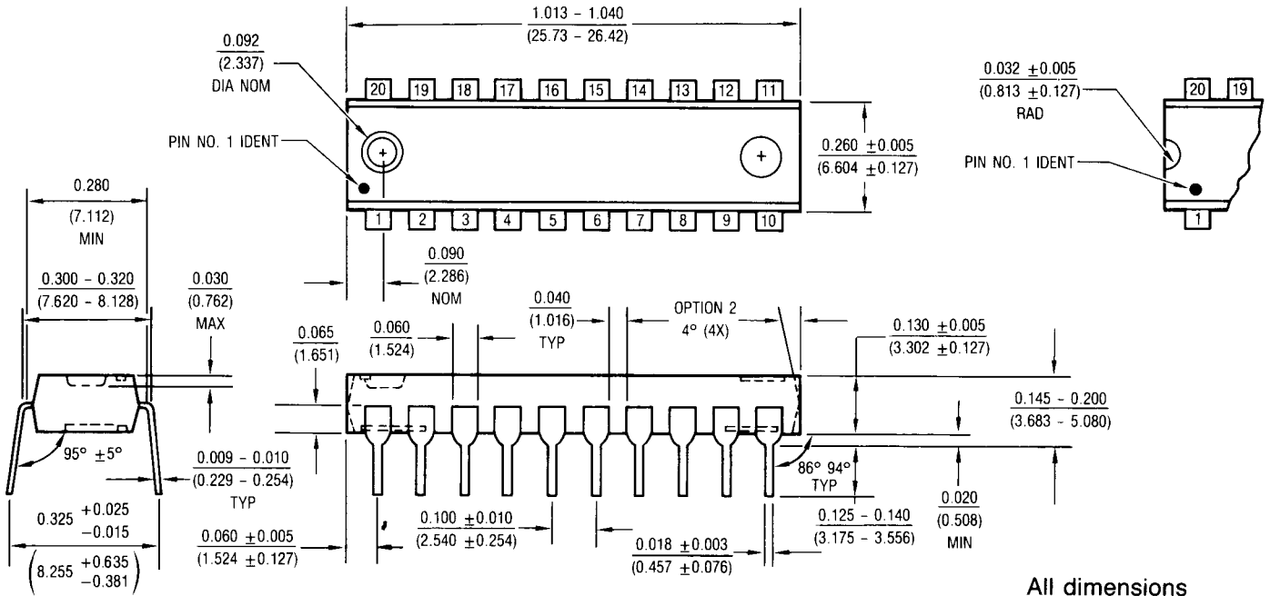
20-Lead Molded DIP Package
