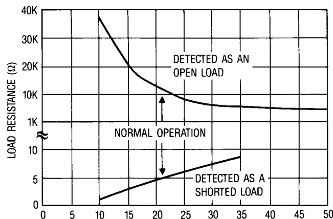
Fig. 23 — Load Resistance Detected as Errors
