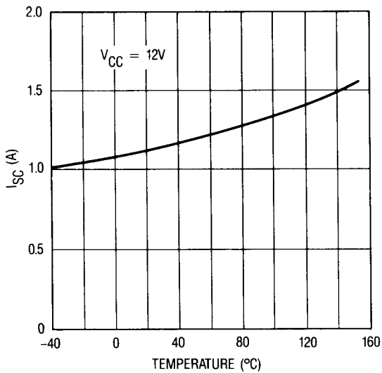
Fig. 3 — Short Circuit Current vs. Temperature
