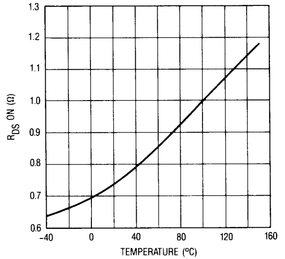
Fig. 2 — Switch ON Resistance vs. Temperature
