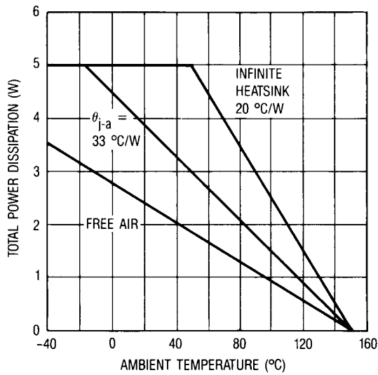
Fig. 13a — Maximum Power Dissipation vs. Ambient Temperature
