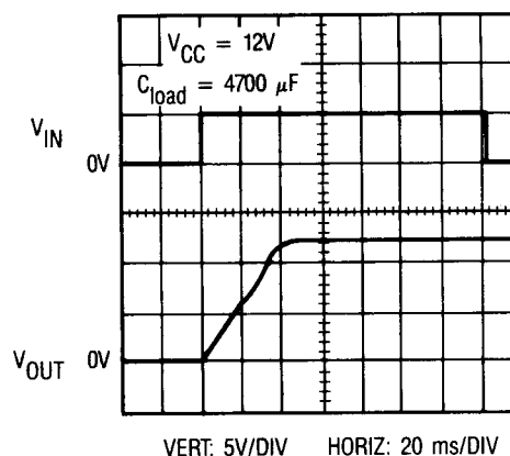
Fig. 20 — Driving a Large Capacitive Load
