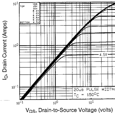
Fig 2. Typical Output Characteristics, T_C=150^\circ C
