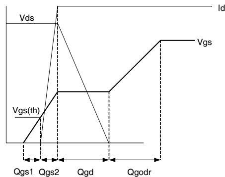
Fig 16. Gate Charge Waveform
