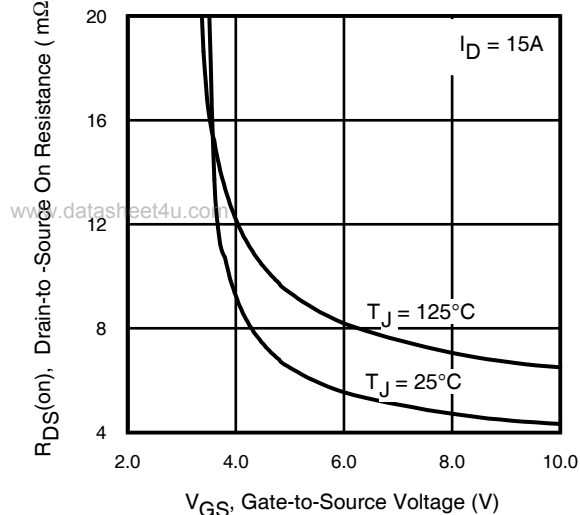
Fig 12. On-Resistance Vs. Gate Voltage
