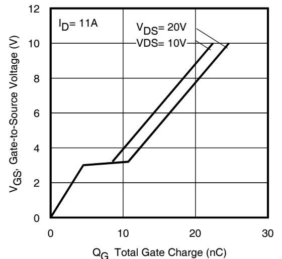
Fig 6. Typical Gate Charge vs. Drain-to-Source Voltage www.irf.com
