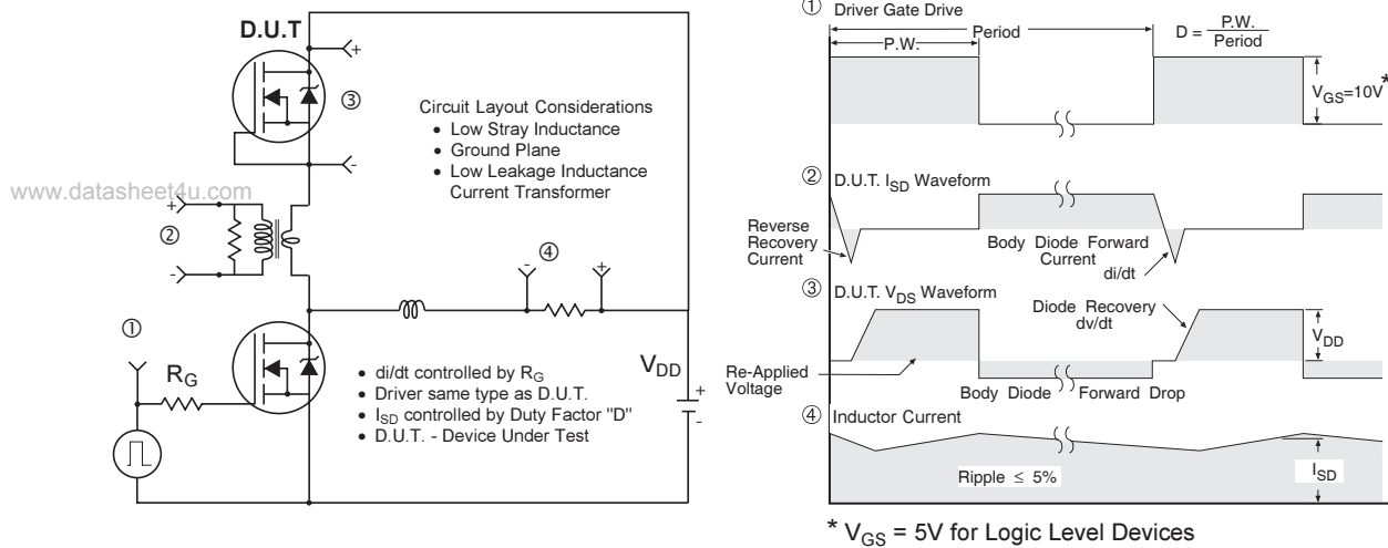
Fig 17. Diode Reverse Recovery Test Circuit for N-Channel HEXFET® Power MOSFETs
