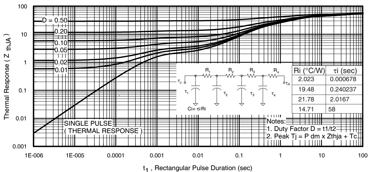
Fig 11. Maximum Effective Transient Thermal Impedance, Junction to Ambient
