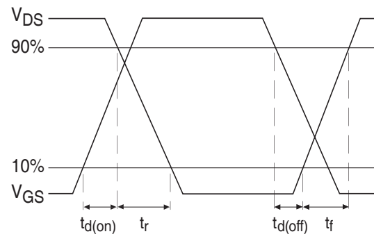
Fig 17b. Switching Time Waveforms www.DataSheet4U.com www.irf.com
