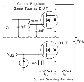
Fig 27a&b. Basic Gate Charge Test Circuit and Waveform
