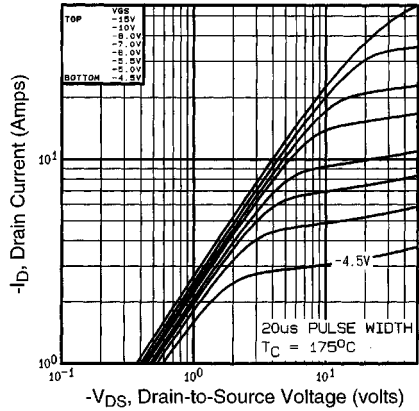
Fig 2. Typical Output Characteristics, T_C=175^\circ C
