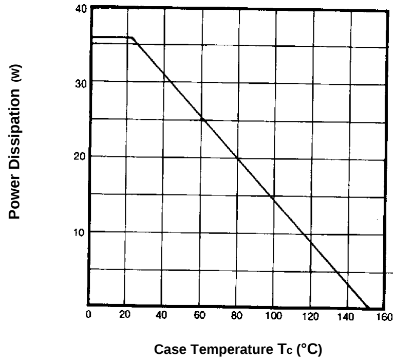
Fig.14-Power Vs. Temperature Derating Curve
