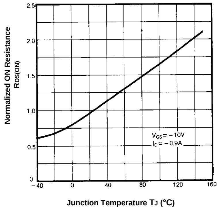
Fig.9- Normalized On-Resistance Vs. Temperature
