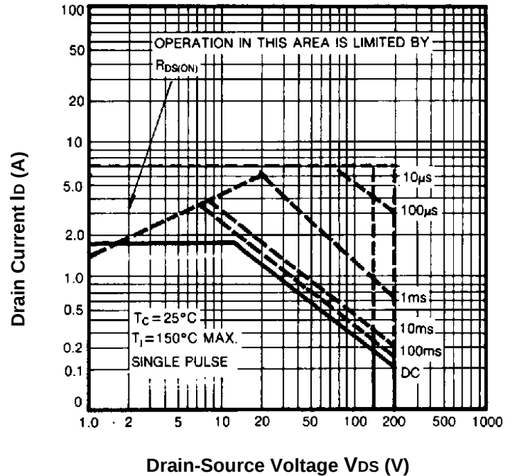
Fig.4- Maximum Safe Operation Area
