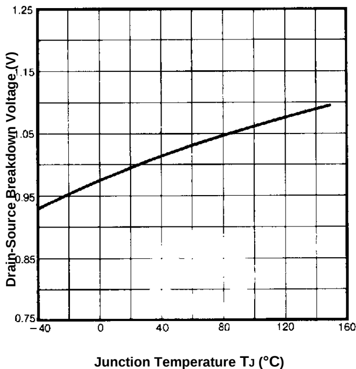
Fig.8- Breakdown Voltage Vs. Temperature
