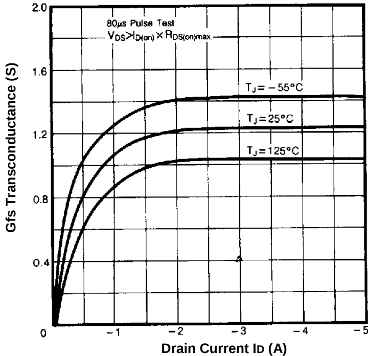
Fig.6- Typical Transconductance Vs. Drain Current
