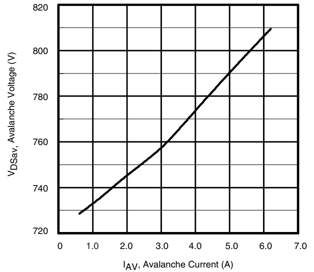
Fig. 12d - Typical Drain-to-Source Voltage vs. Avalanche Current
