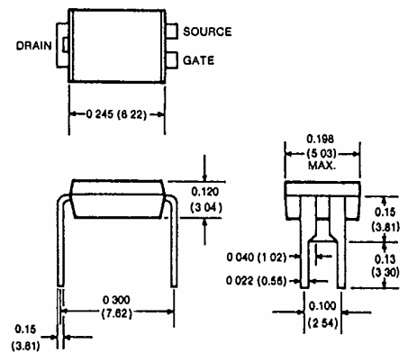
CASE STYLE 4-PIN DIP DIMENSIONS ARE IN INCHES AND (MILLIMETERS)
