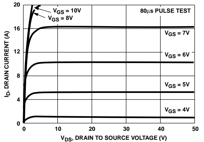
FIGURE 5. OUTPUT CHARACTERISTICS
