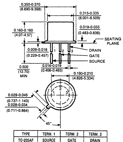
CASE STYLE TO-205AF (TO-39) DIMENSIONS ARE IN INCHES AND (MILLIMETERS)
