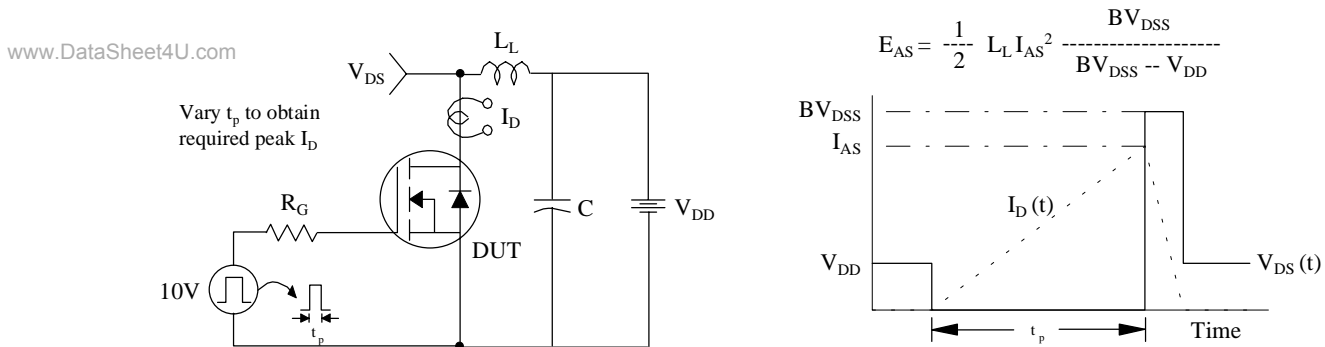
Fig 14. Unclamped Inductive Switching Test Circuit & Waveforms
