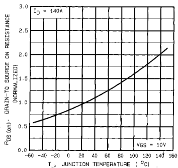
Fig 4. Normalized On-Resistance Vs. Temperature
