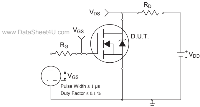
Fig 23a. Switching Time Test Circuit
