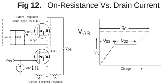
Fig 14a&b. Gate Charge Test Circuit and Waveform
