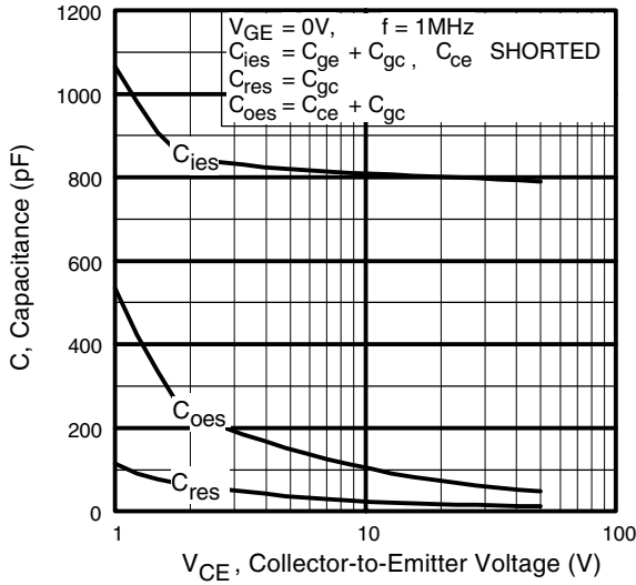
Fig. 7 - Typical Capacitance vs. Collector-to-Emitter Voltage DataSheet4U.com
