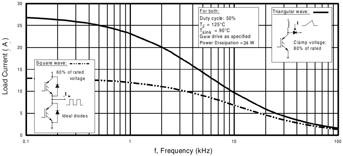
Fig. 1 - Typical Load Current vs. Frequency (Load Current = I_{RMS} of fundamental) DataSheet4U.com
