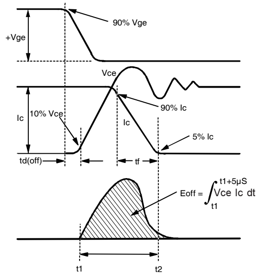
Fig. 18b - Test Waveforms for Circuit of Fig. 18a, Defining E_{off} , t_{d(off)} , t_{rf}
