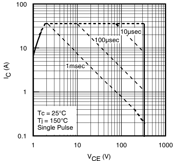
Fig 12. Forward Bias Safe Operating Area www.DataSheet4U.com www.irf.com
