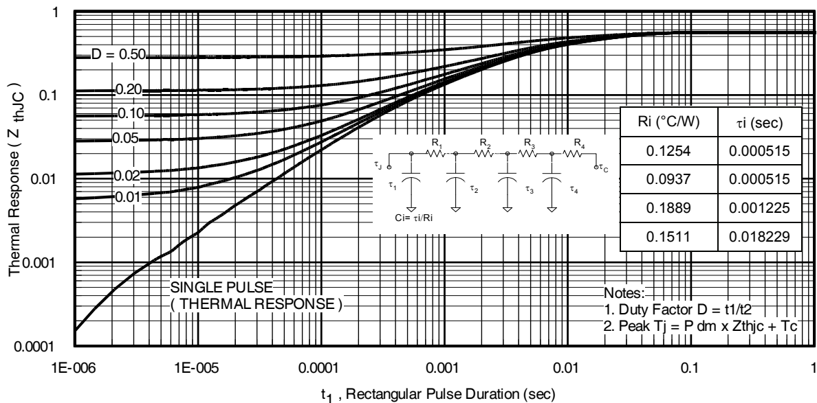
Fig. 26 - Maximum Transient Thermal Impedance, Junction-to-Case (DIODE)
