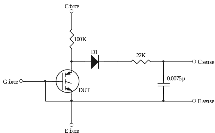
Fig.C.T.6 - BV CES Filter Circuit www.DataSheet4U.com
