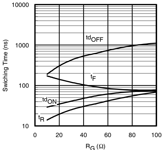
Fig. 16 - Typ. Switching Time vs. R_G T_J = 175^\circ C ; L = 680\mu H ; V_{CE} = 600V , I_{CE} = 20A ; V_{GE} = 15V
