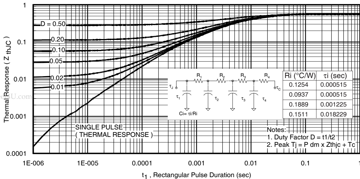
Fig. 25. Maximum Transient Thermal Impedance, Junction-to-Case (DIODE) www.DataSheet4U.com
