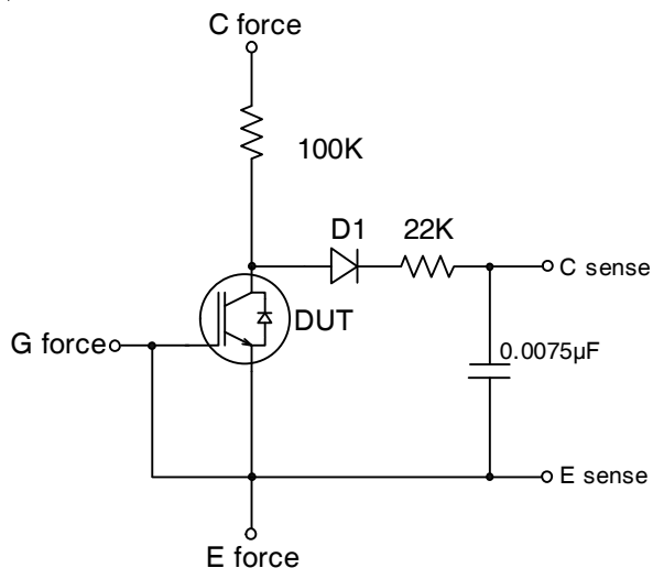
Fig.C.T.4 - BVCE Filter Circuit
