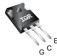
IRG8P15N120KDPbF TO-247AC
