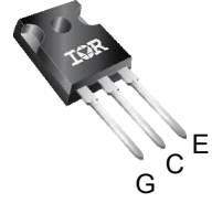
IRG8P25N120KD-EPbF TO-247AD
