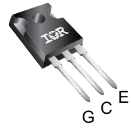
IRG8P40N120KD-EPbF TO-247AD
