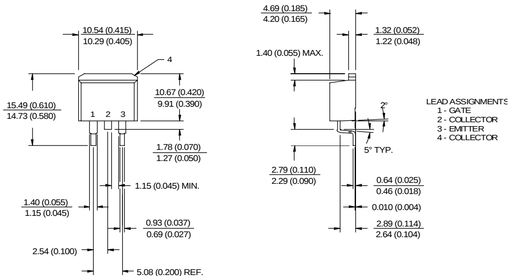
OUTLINE SMD-220 Dimensions in Millimeters and (Inches)
