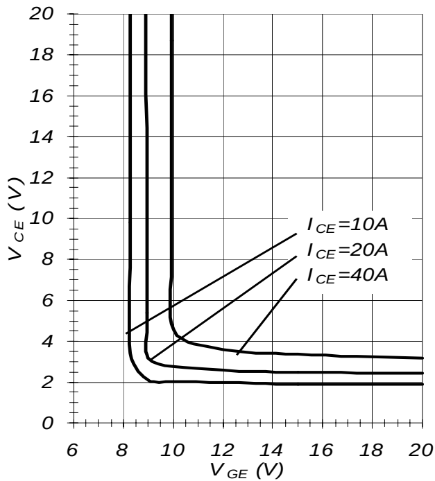
Fig. 8 - Typical V_{CE} vs V_{GE} T_j = -40^\circ\text{C}
