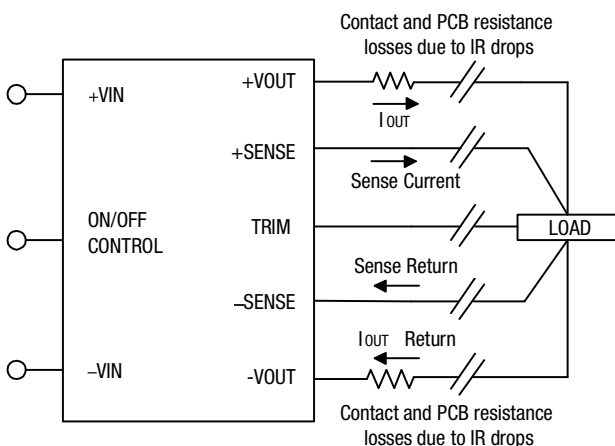
Figure 5 Remote Sense Circuit Configuration
