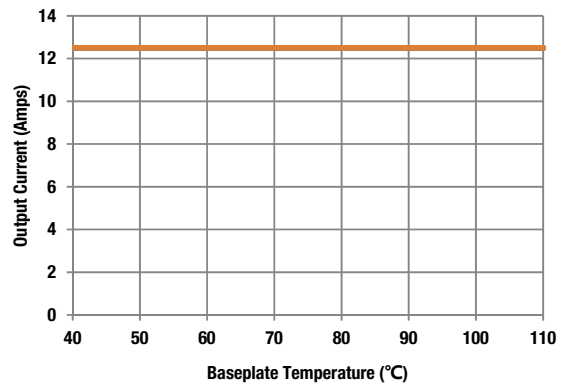
Thermal Derating vs. Baseplate temperature
