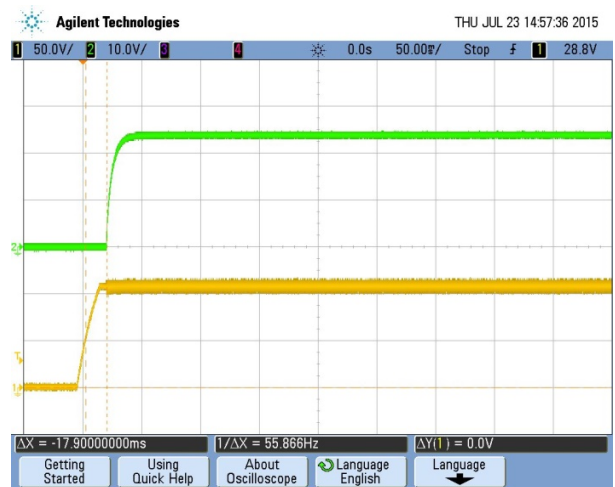
Turn-on transient at full load current (50 mS/div, Top Trace: Vout, 10V/div; Bottom Trace: Vin, 50V/div)
