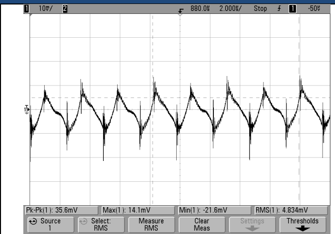
Ripple and Noise @25°C
