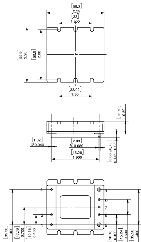
SLOTTED / FLANGED BASEPLATE
