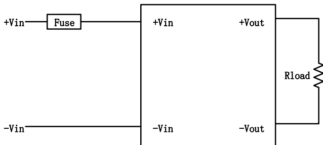
Figure 2. Input Fusing
