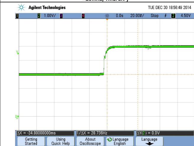
Start-up into a Pre-bias Load@25°C
