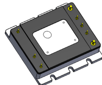
Slotted / Flanged Baseplate DOSA Pins / Pinout Pin Diameter: 0.040 / 0.080
