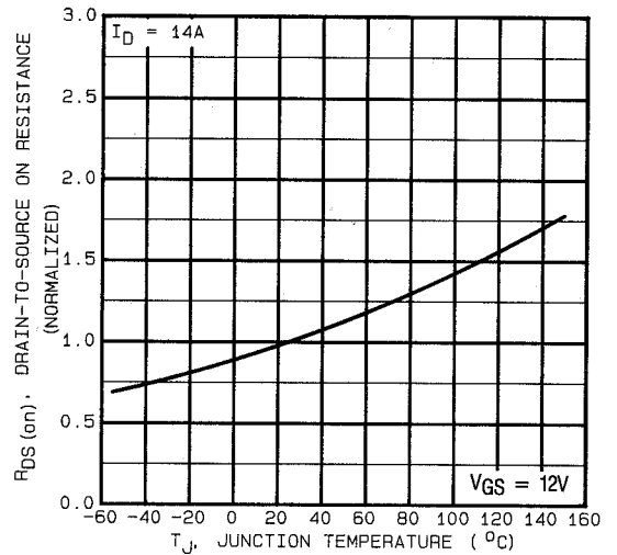
Fig 20. Normalized On-Resistance
