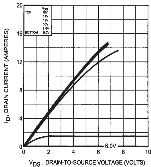
Fig 12. Typical Output Characteristics Post-Irradiation 300K Rads (Si)
