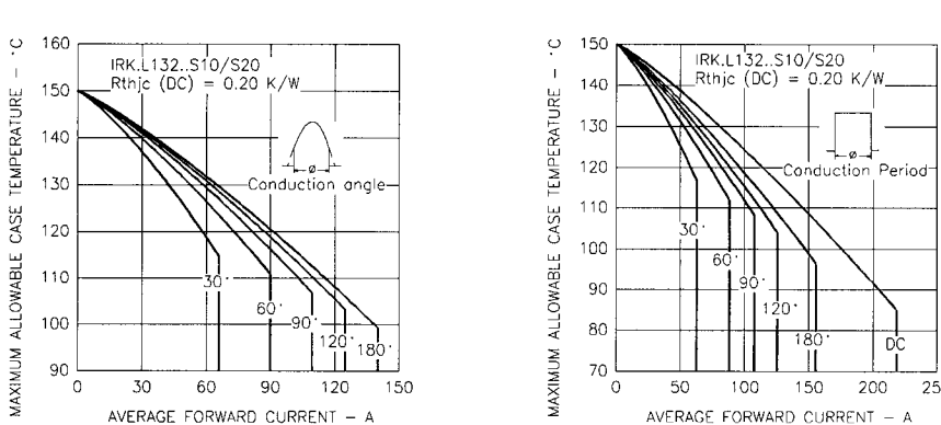
Fig. 1 - Current Ratings Characteristics
