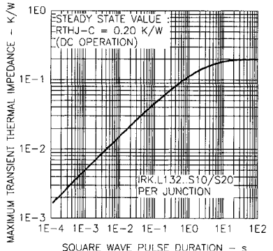
Fig. 8 - Thermal Impedance Characteristics
