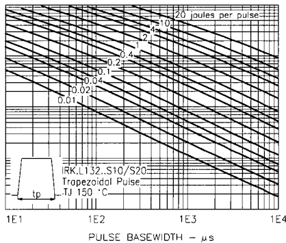
Fig. 13 - Maximum Forward Energy Power Loss Characteristics
