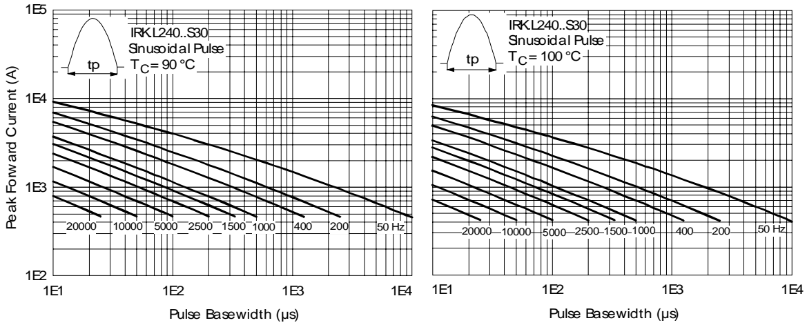
Fig. 25 - Frequency Characteristics
