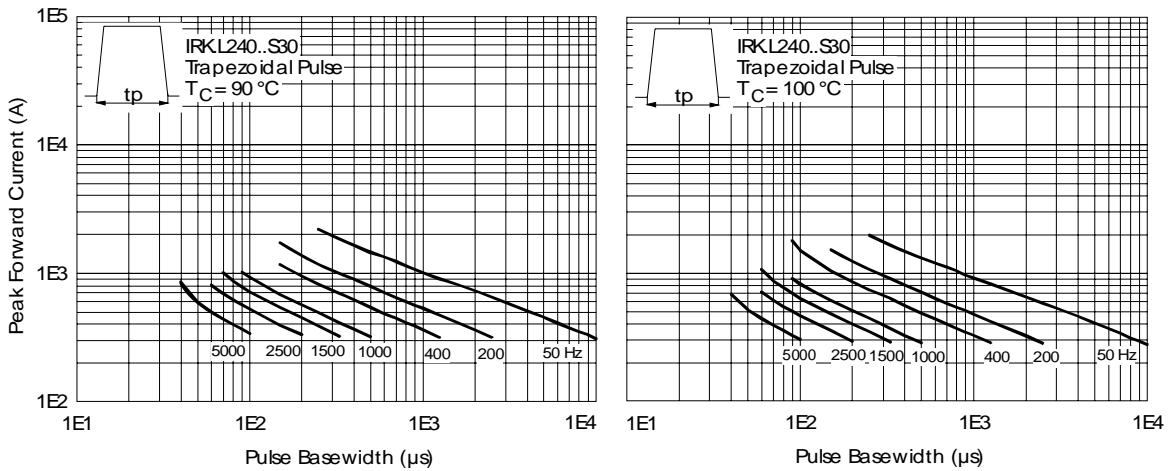
Fig. 26 - Frequency Characteristics
